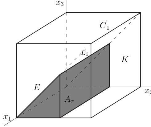
Figure 3.1: The counterexample
