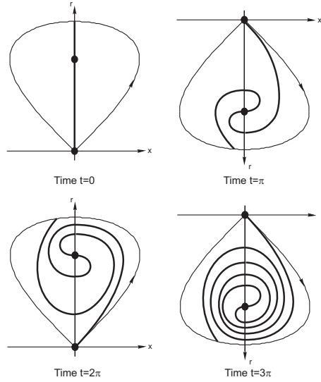
Figure 5.2: The evolution of the set S_\varphi for some values of the time.
