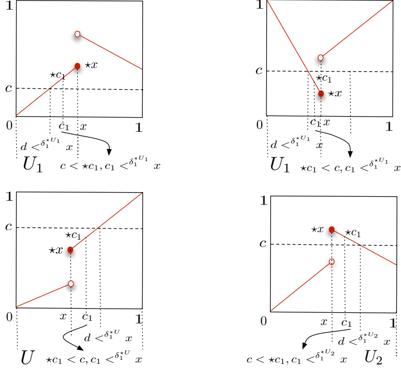
Figure 4.2: Examples for the rule C_1^U .
