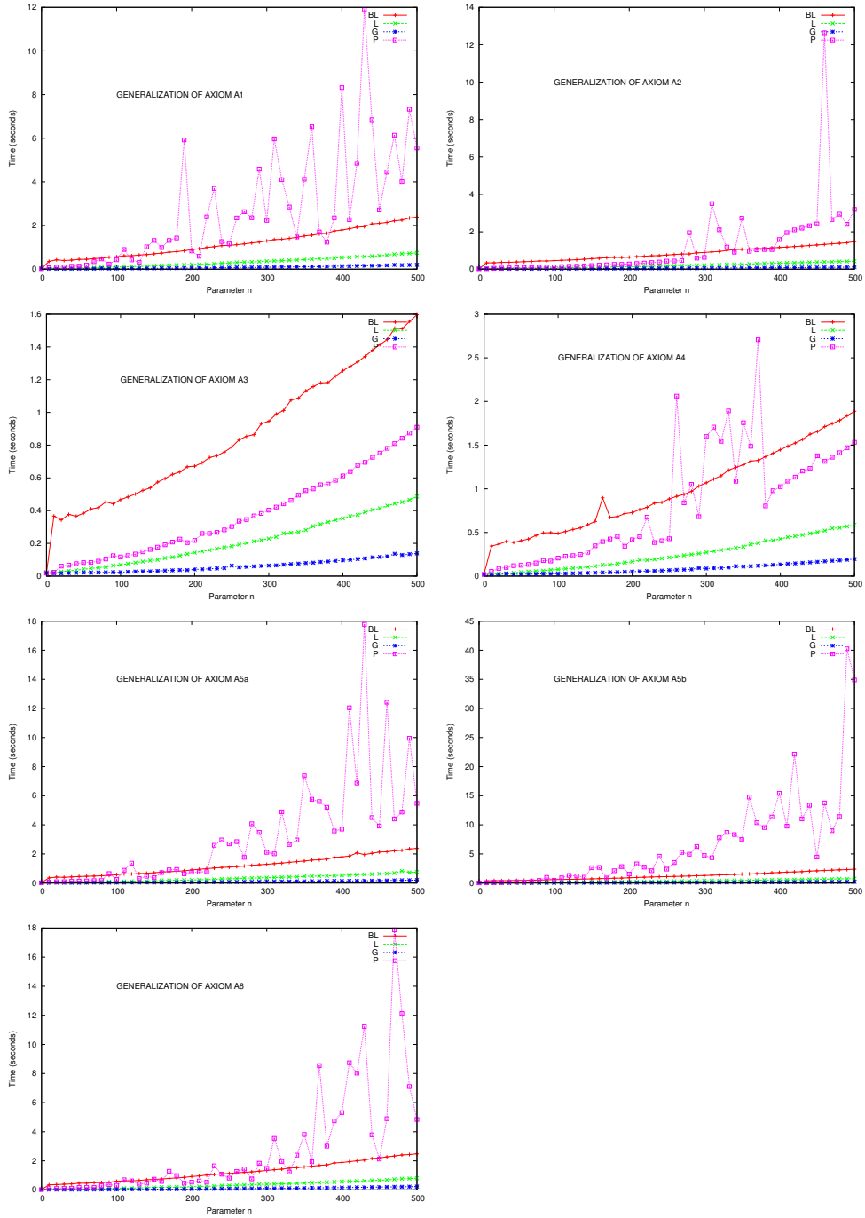
Figure 11.1: Generalizations of BL-axioms given in (11.1).
