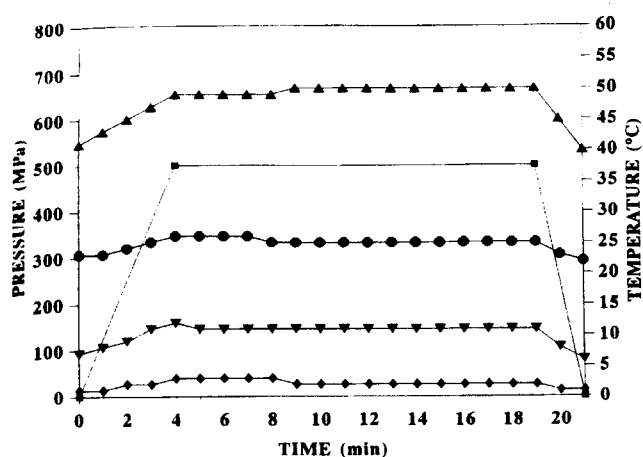
Figure 1. Variation of the chamber water temperature as a function of time during treatment at 2°C (♦), 10°C (▼), 25°C (●), and 50°C (▲) and at 500 MPa of pressure (■).
