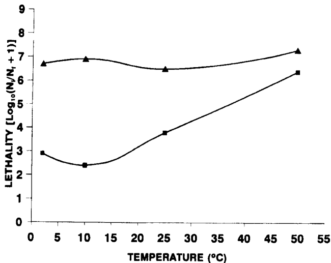
Figure 6. Lethality [ \log_{10}(N_i/N_f + 1) ] of high hydrostatic pressure as a function of temperature during 5 min of treatment at 400 MPa of ovine milk that had been inoculated with Pseudomonas fluorescens 378 CECT (▲) and Escherichia coli 405 CECT (■).
