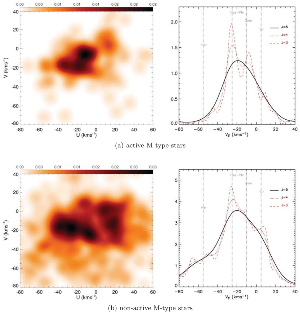
Figure 7.3: Velocity distribution for different chromospheric activity. Density field in the U - V plane obtained by WD with J = 4 (left) and density field for the V_{\beta} component with different values of J (right) for the subsamples of (a): active (182 stars) and (b): non-active (681 stars).
