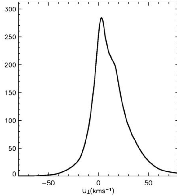
Figure 6.5: Kinematic edge line. Density field in the direction perpendicular to the edge line ( U_{\perp} ) for the whole observational sample ( J_{plateau} = 4 ).
