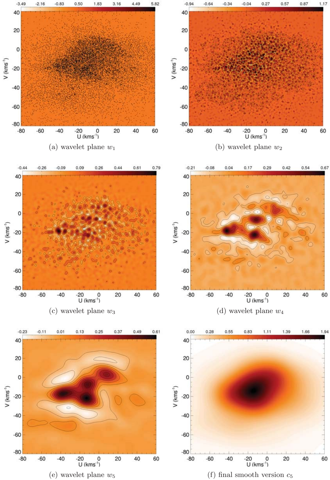
Figure 4.3: Wavelet planes. WT in the U - V plane: wavelet planes w_i together with the final smooth version c_5 .
