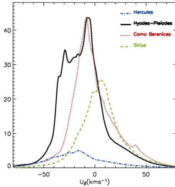
Figure 6.6: Kinematic distribution along the branches. Density field for the U_{\beta} component for each of the four branches ( J_{plateau} = 4 ).
