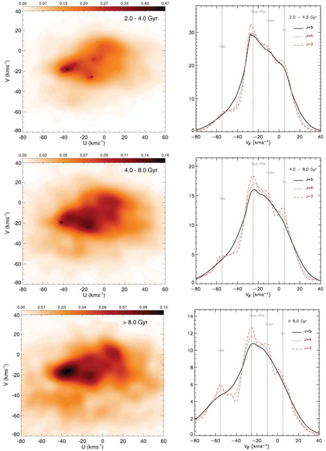
Figure 7.2: Velocity distributions for different ages (II) . Left column: Density field in the U - V plane obtained by WD with J = 4 for subsamples of different ages (in Gyr): 2.0-4.0 (3917), 4.0-8.0 (2561) and >8.0 (2053). Right column: Density field for the V_\beta component with different values of J of the WD: 3, 4 and 5.
