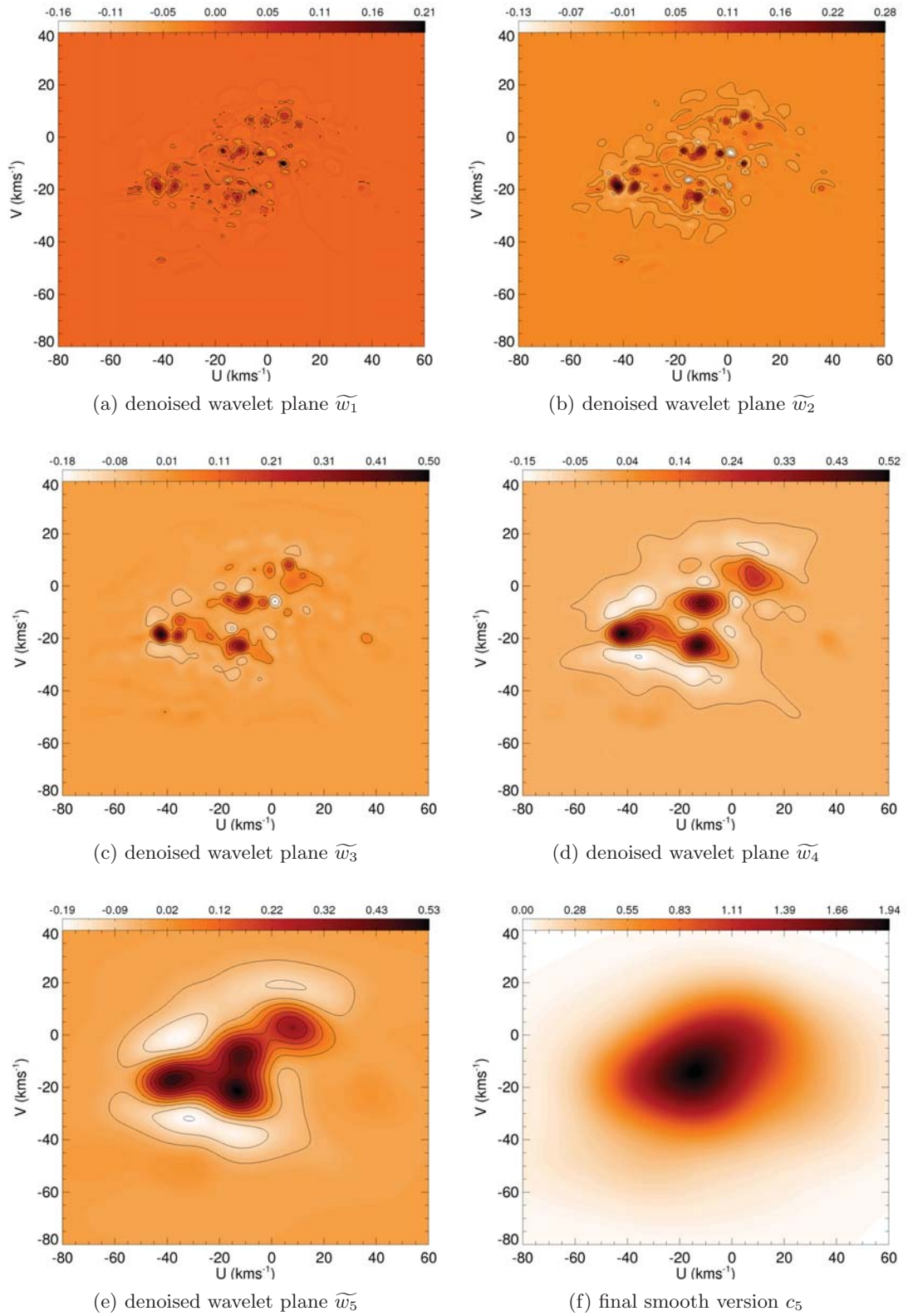
Figure 4.5: Denoised wavelet planes. WD of the wavelet planes \tilde{w}_i together with the final smooth version c_5 which does not change.
