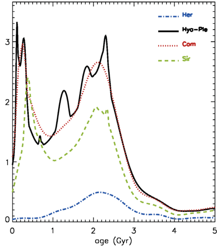
Figure 7.5: Age distribution of the branches. Density of stars in each branch as a function of age for stars with \epsilon_{age} \leq 30\% (223, 1195, 1078 and 806 stars in the Hercules, Hyades-Pleiades, Coma Berenices and Sirius branches respectively).
