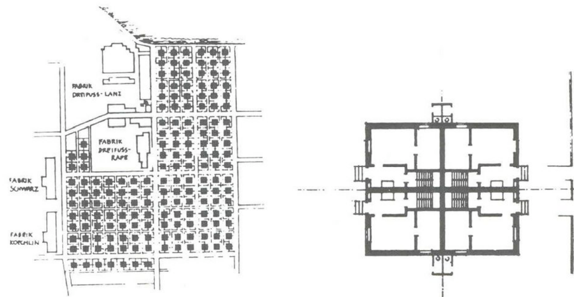
Image, Site Plan and Detailed Floorplan
