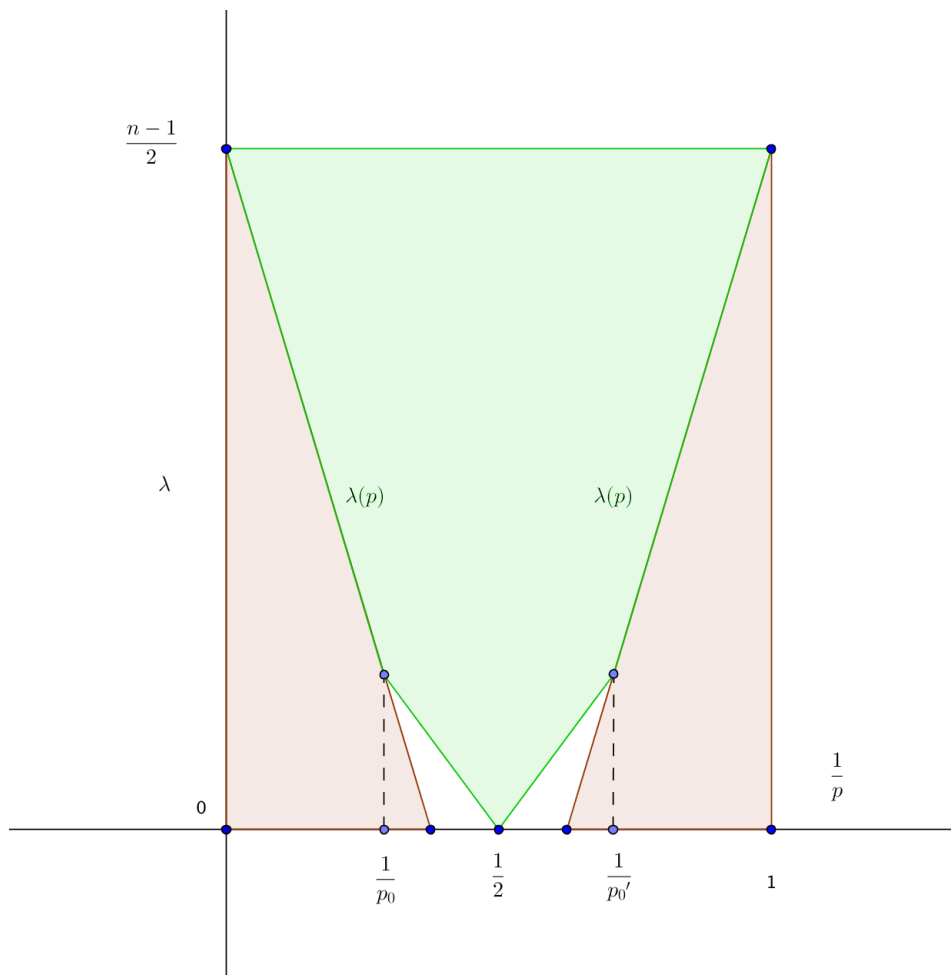
Figure 3.2: Current state of the Bochner-Riesz conjecture for n \geq 3 , with p_0 as in (3.12).
