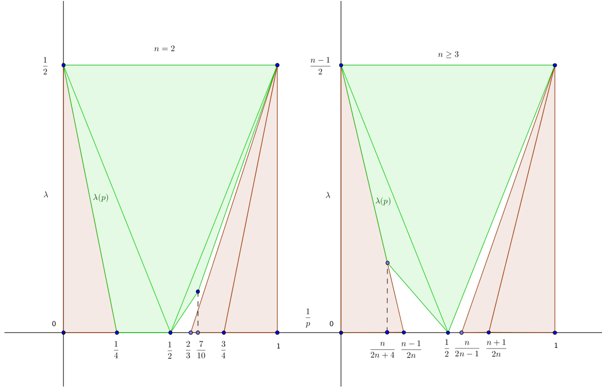
Figure 3.3: Current state of the Maximal Bochner-Riesz conjecture.
