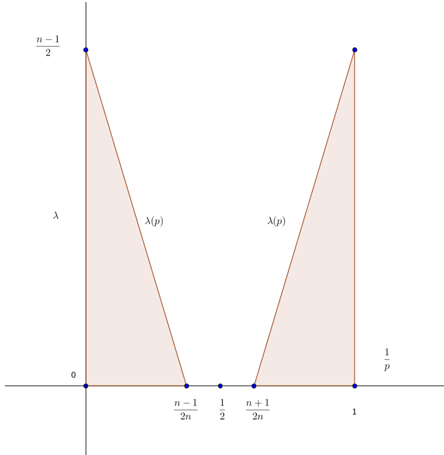
Figure 3.1: B_\lambda should be bounded on L^p(\mathbb{R}^n) for (1/p, \lambda) outside the shaded region.
