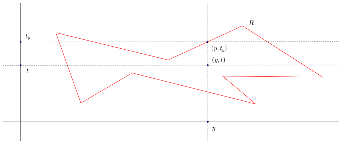
Figure 4.1: Idea of the definition of t_y .
