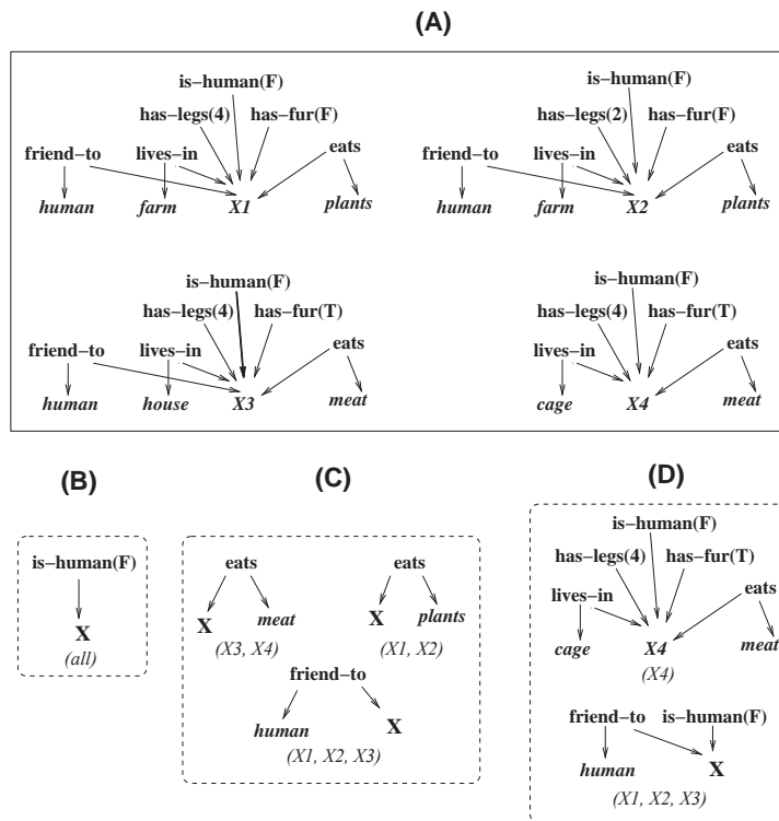
Fig. 1. Analogy-based generalization. This figure shows a set of exemplars representing individual animals encountered by a child (A) and several possible generalization-sets representing categorizations of these animals (B–D), where both exemplars and generalizations are represented as predicate-structures. This figure demonstrates that different generalization-sets are not equally useful. Some are too small to be informative (B), some are composed of generalizations that do not summarize distinct subsets of the given exemplars (C), and some are too highly detailed, and thus processed inefficiently (generalization-set equal to (A); not shown). Part (D) shows a generalization-set that strikes a reasonable balance wrt informativity, distinctness, and compactness.
