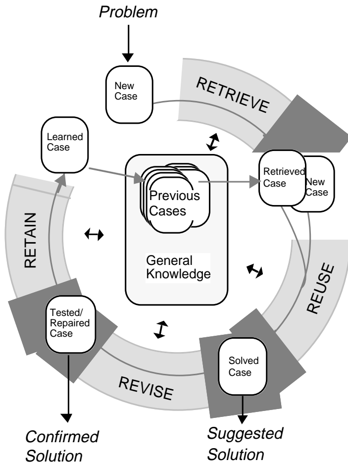
Figure 19: Overview of the traditional case-based reasoning cycle (Aamodt and Plaza, 1994). Figure 1. The CBR Cycle
