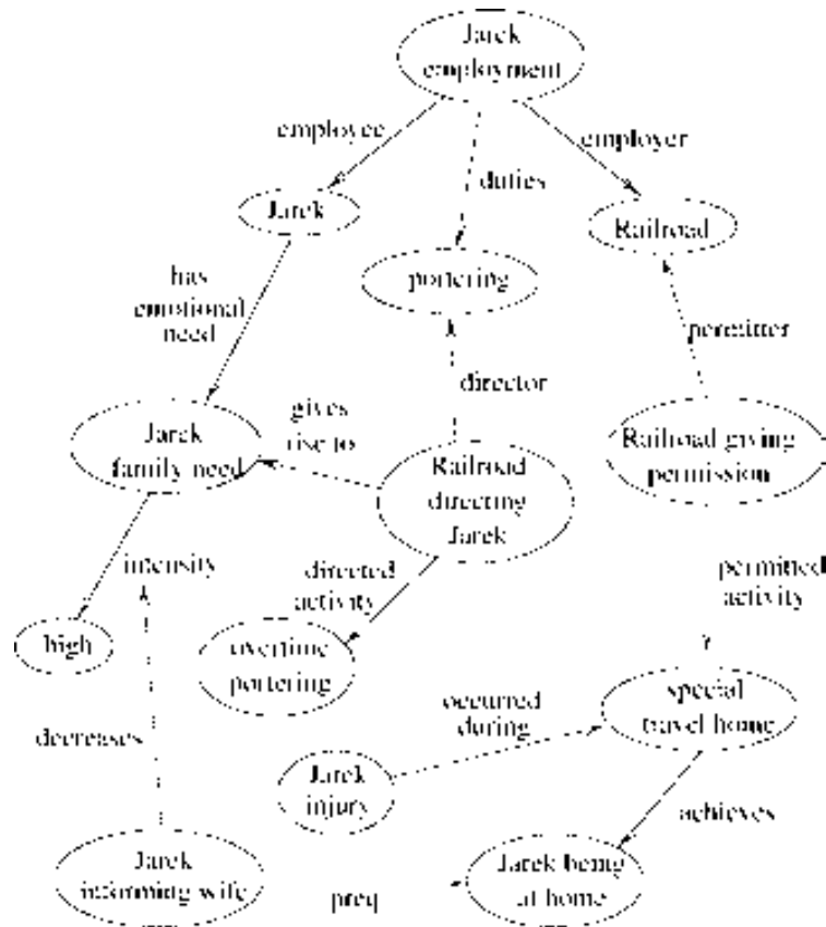
Figure 64: Representation of the facts in Jarek's Case , concerning the compensation of an injured railroad employee, in the GREBE system of
