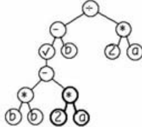
Figure 27: The crossover operation in genetic programming with identical parents. The bold sections are swapped to create the offspring (Fernandez, 2013).
