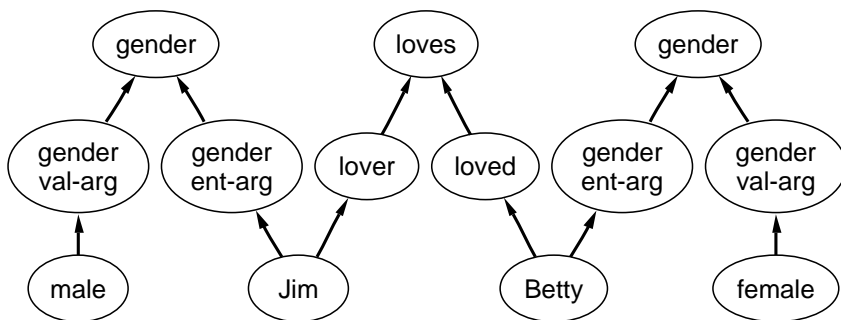
Fig. 1. The analog “Jim loves Betty” can be represented in predicate calculus as \text{loves}(\text{Jim}, \text{Betty}) , \text{gender}(\text{Jim}, \text{male}) , \text{gender}(\text{Betty}, \text{female}) or by the directed graph shown in the figure.
