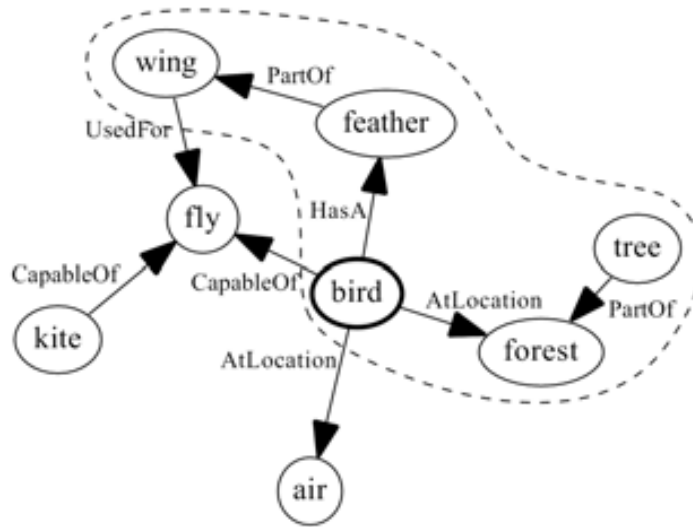
Figure 36: Commonsense crossover type I (subgraph crossover). Parent 1, centered on the concept bird.
