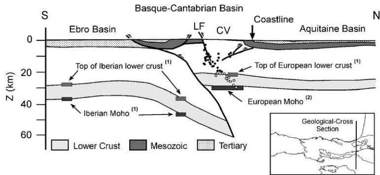
Fig. 8. Cartoon of the crustal structure, derived from seismic and 3D gravity and magnetic modelling (Pedreira, 2004; Pedreira et al., submitted for publication) along the trace of the N–S section B–B' with the earthquake hypocentres superimposed. Constraints on the position of the Moho and the top of the lower crust are marked at the intersection with available seismic refraction and receiver function profiles: (1): Pedreira et al. (2003) and (2): Gallart et al. (1981), Díaz et al. (2003). LF: Leiza Fault. CV: Cinco Villas Massif.
