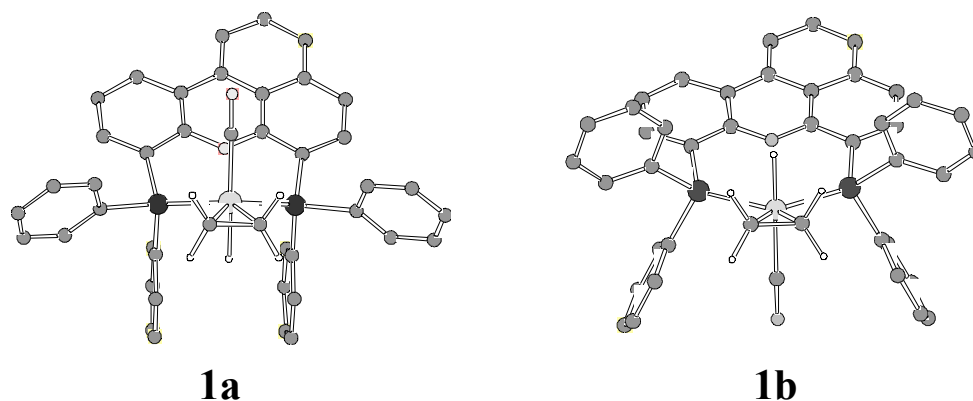
Figure 6.2. IMOMM structures of HRh(alkene)(CO)(benzoxantphos) isomers 1a and 1b . The hydrogen atoms of xantphos ligands are omitted for clarity.
