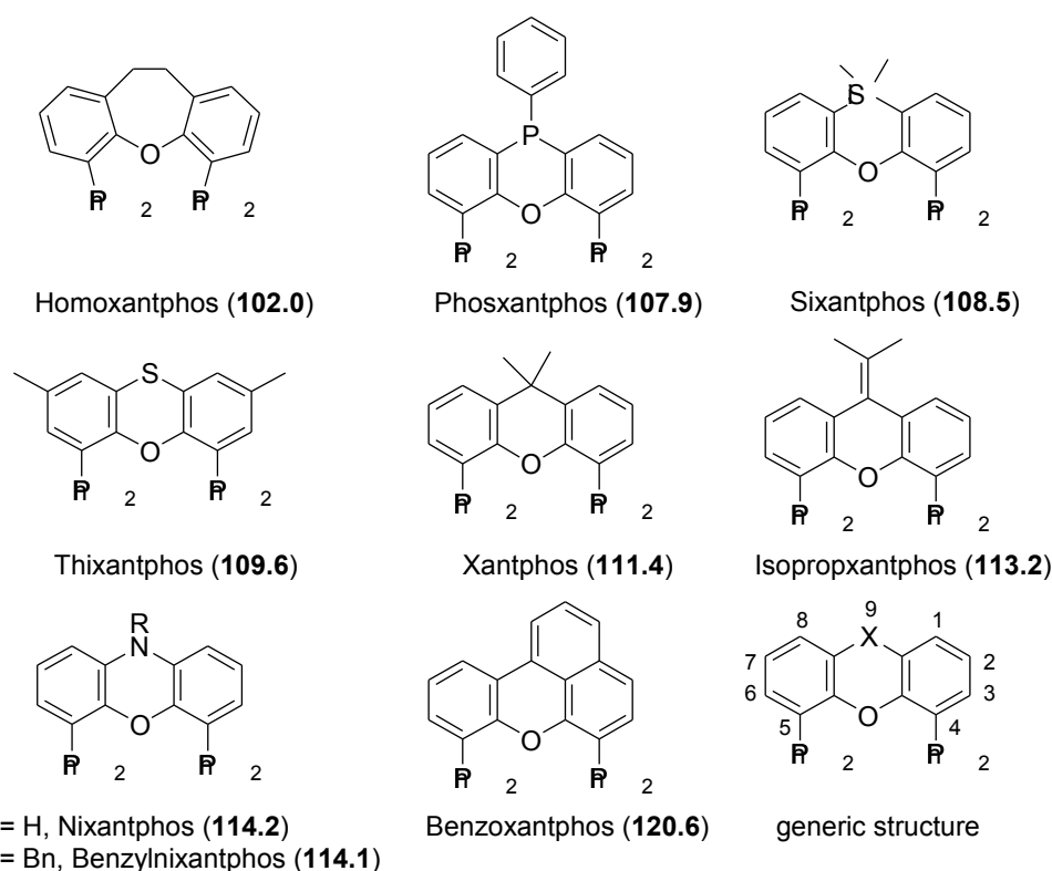
Figure 6.1. Schematic representation of the xantphos ligand family. The natural bite angle is given in parentheses.
