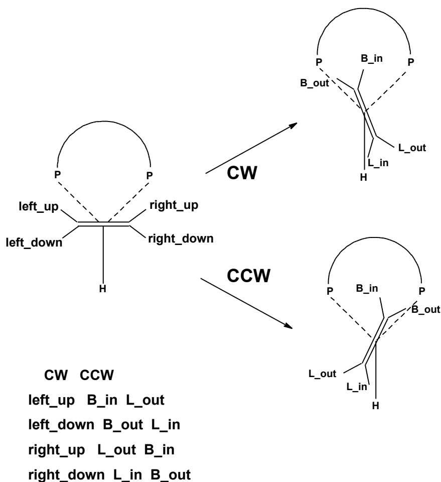
Figure 6.3. Definition of the eight possible reaction paths for alkene insertion from the key equatorial-equatorial pentacoordinate intermediate.
