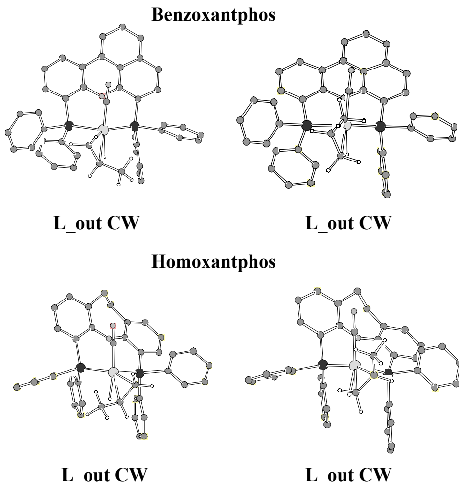
Figure 6.4. IMOMM TS structures of some representative isomers for propene insertion on benzo- and homoxantphos systems. TS's are presented as in Figure 6.3 (front view), and the hydrogen atoms of xantphos ligands are omitted for clarity.
