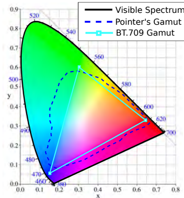
Figure 3.12: BT.709 gamut in the CIE xy chromaticity diagram.
