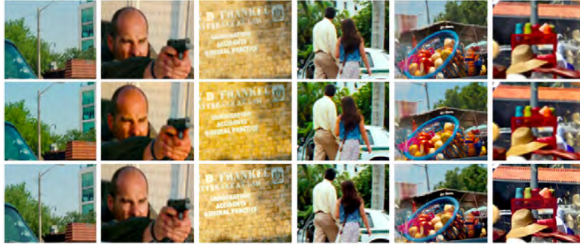
Figure 5.18: Comparison of GEAs, details from Fig. 5.17; top row, ground truth; middle row, output of Same Drive Signal algorithm [Laird et al., 2009]; bottom row, output of our GE method. The results of the SDS algorithm [Laird et al., 2009] are highly saturated and off from the ground truth. See the reproduction of sky, trees, skin tone, wall, clothes, fruit bucket and hat.
