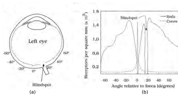
Figure 2.7: Distribution of photoreceptors across the human retina: (a) visual angles relative to the fovea, (b) concentration of cones and rods in the fovea. Figure is taken from [Wandell, 1995].
