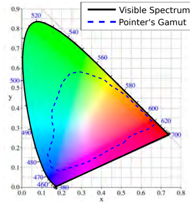
Figure 3.11: Pointer's gamut in the CIE xy chromaticity diagram.
