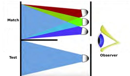
Figure 2.19: Color matching experiment.
