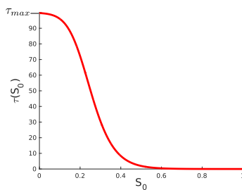
Figure 7.1: Logistic function.
