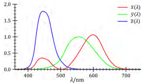
Figure 2.21: Color matching functions \bar{x}(\lambda) , \bar{y}(\lambda) and \bar{z}(\lambda) . Image from [Wikipedia, 2007].
