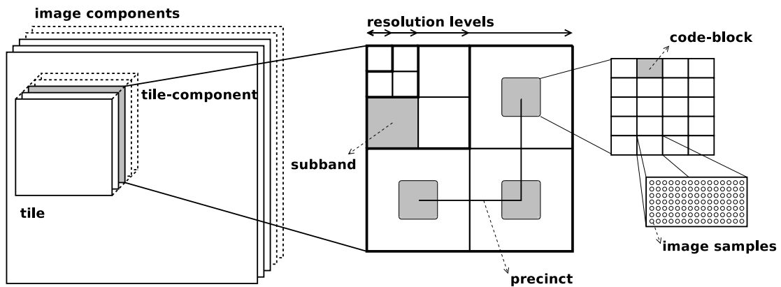
Figure 2.5: The JPEG2000 partitioning system.
