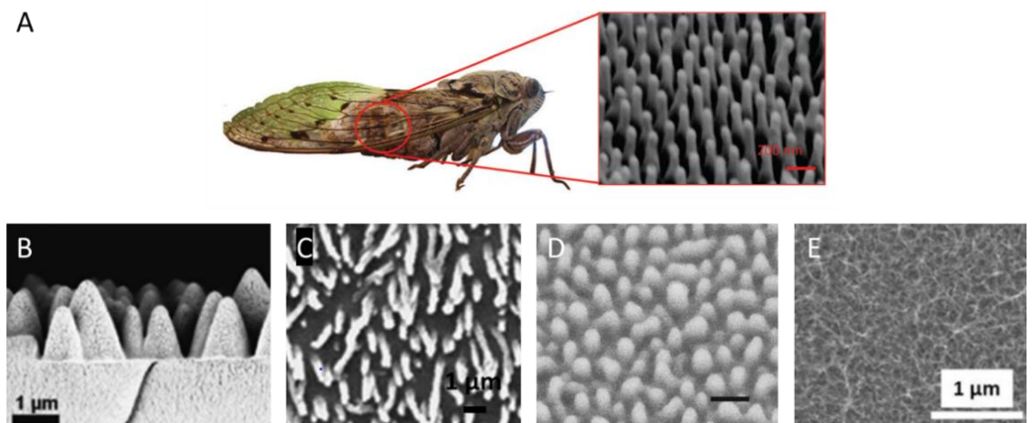
Figure I. 3. Field emission scanning electron microscopy images of different bio-inspired nanostructured surfaces. Image of bio-nanopyllars in cicada wings 43,50 (A), to inspire the modification of different substrates with polymer micro-cones or microneedles fabricated using a templating method 50 (B), titanium nanotubes grown via anodic oxidation 50 (C), nanopyllars fabricated by UV nano-replication technology 44 (D) or titanium nanowires by hydrothermal manufacture process (E) 54 . Red bar: 200 nm, black bars: 1 \mu\text{m} . Figure extracted and modified from previously cited works with academic purposes.
