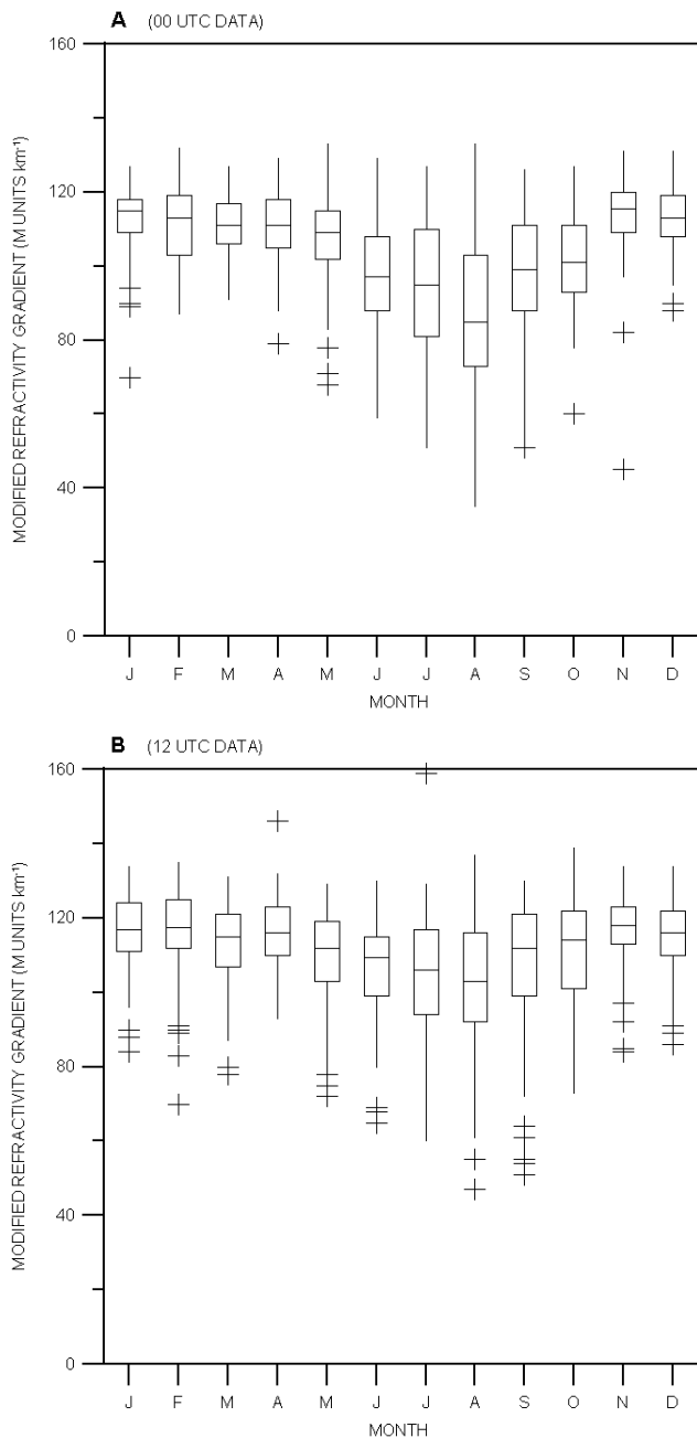
Fig. 3. Box whisker plot showing the first, second (median) and third quartile and outlier points of modified refractivity vertical gradient for the first kilometer above ground level in Barcelona for each month: (a) 00:00 UTC data and (b) 12:00 UTC data.
