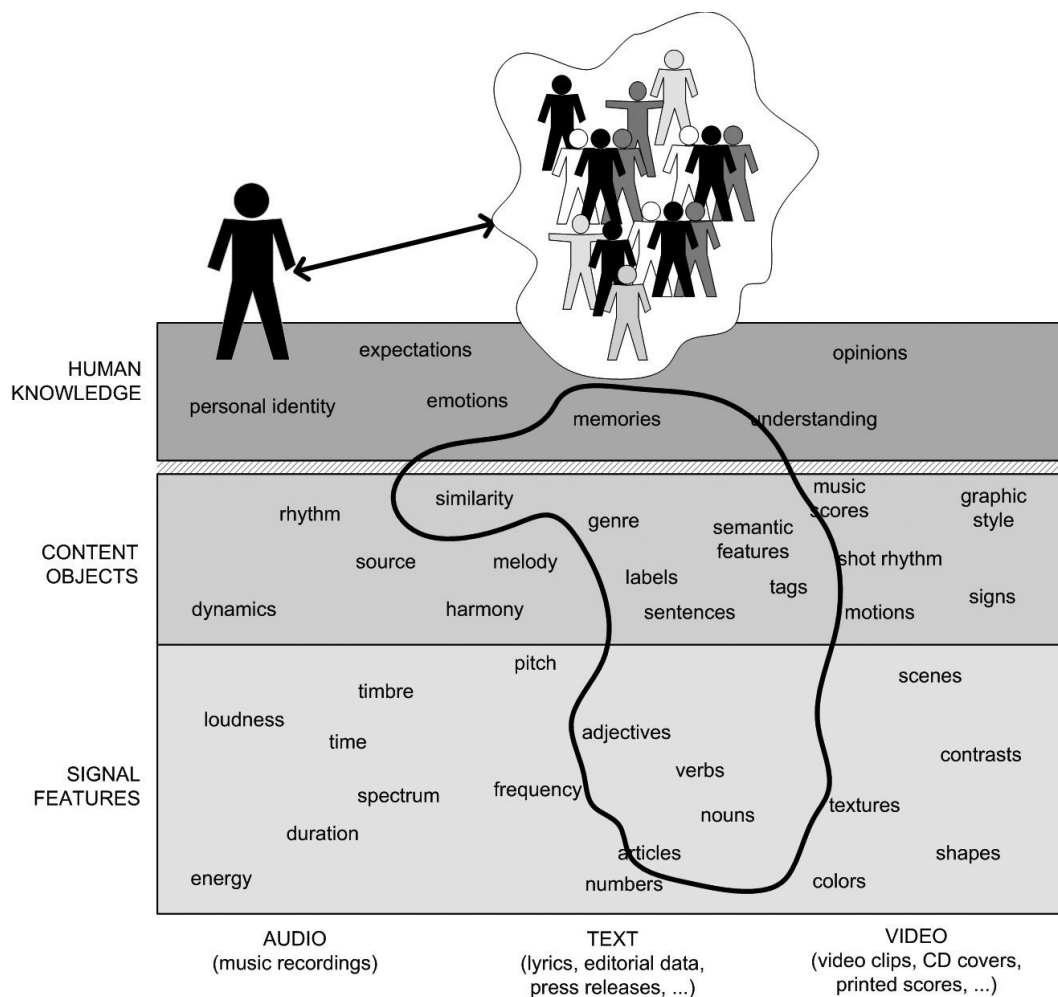
Figure 3.3: Editorial metadata and the music information plane.
