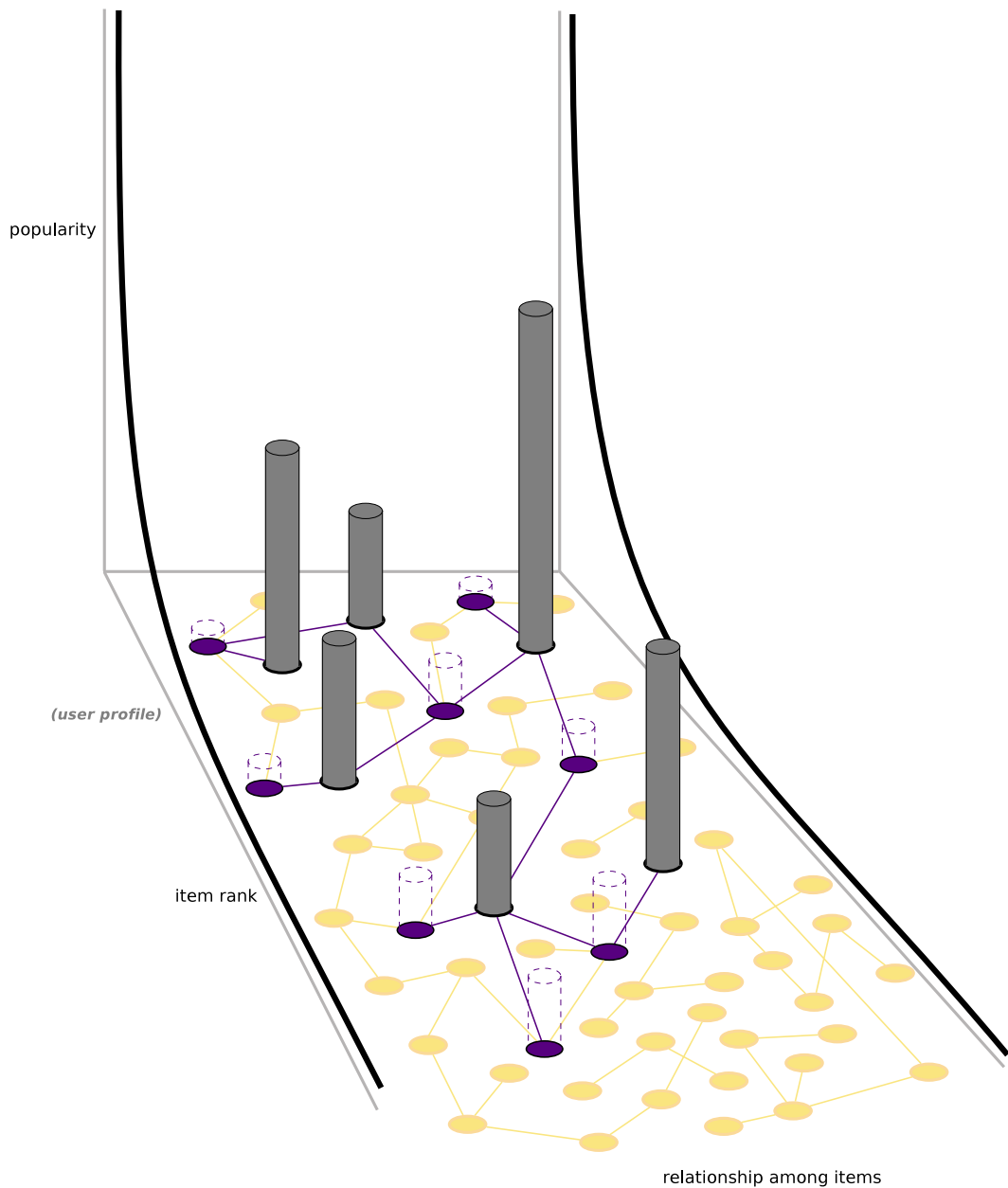
Figure 4.9: (best seen in colour) A 3D representation of the Long Tail. It adds another dimension; the similarities among the items, including the representation of a user profile (in gray). The set of candidate items to be recommended to the user are shown (in violet) and its height denotes the relevance for the user. Candidate items located in the tail part are considered more novel—and, potentially relevant—than the ones in the head region.
