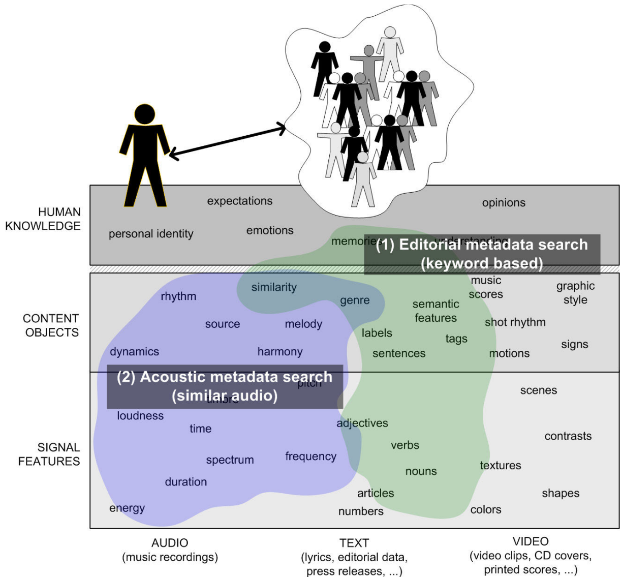
Figure 8.1: SearchSounds makes use of editorial, cultural and acoustic metadata. The system retrieves (1) audio files from a keyword query, as well as (2) a list of (content-based) similar titles.
